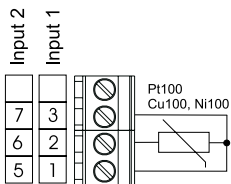
b) RTD inputs in a 3-wire line
