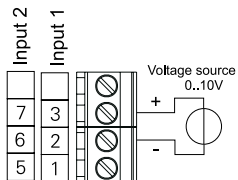
d) Voltage inputs
