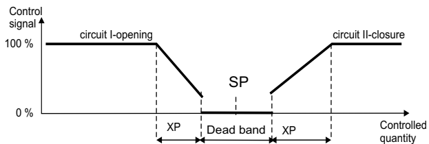
Fig.7.2. Valve control
