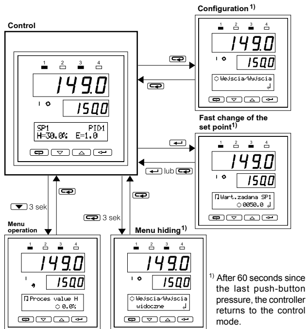
Fig.4.2. Transition diagram between controller operation modes
