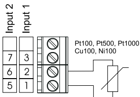
a) RTD inputs in a 2-wire line
