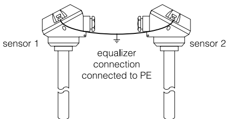
Fig. 3.1. Connection of two sensors.
