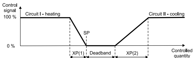
Fig.7.1. Control with two heating-cooling circuits
