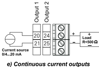
Fig.3.5. Output connections.
