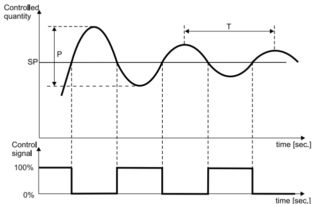
Fig.9.2. Selection of PID parameters through the oscillation method
