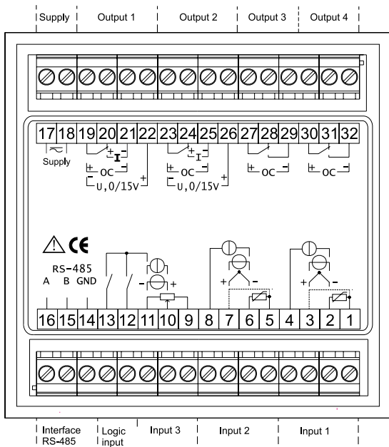
Fig.3.3. Description of the terminal strip.
