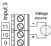
f) Auxiliary voltage input
