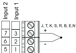
c) Thermocouple inputs
