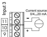
g) Auxiliary current input
