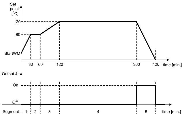
Fig.8.1. Exemplary program of the set point and logic output
