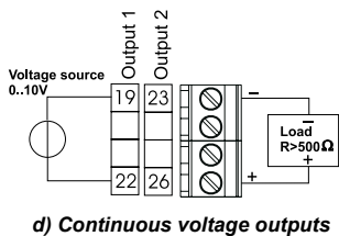
Fig.3.5. Output connections.
