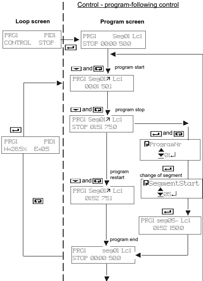
Fig.8.4. Example of program operation control
