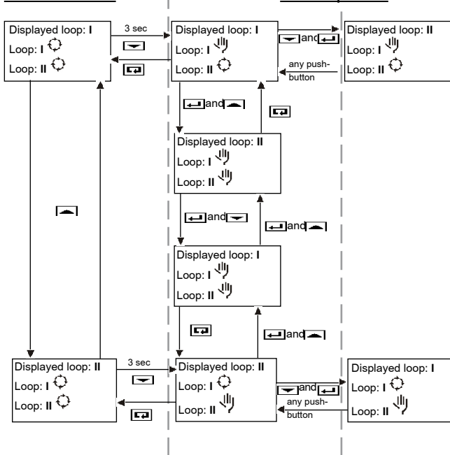
Fig.4.3. Manual control diagram
