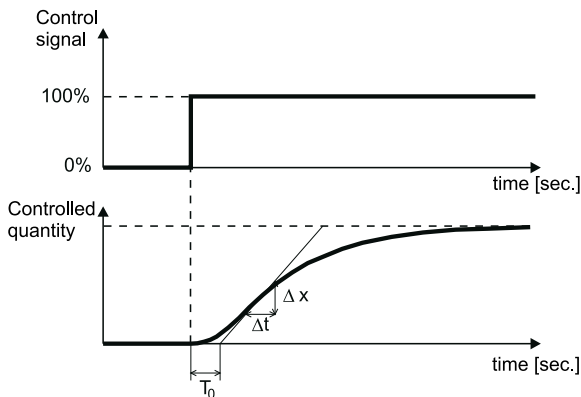
Fig.9.1. Selection of PID parameters through the object identification method
