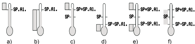
Fig.6.2. Kinds of alarms
