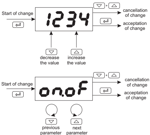
Fig.9. Setting change of numerical and textual parameters.
