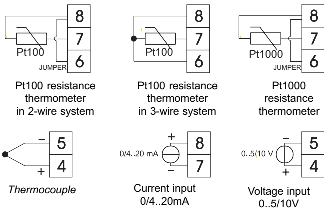
Fig.4. Connection of input signals.
