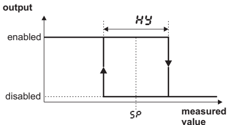
Fig.10. Operation way of the heating type output
