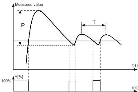
Fig.12. Selection of settings by the oscillation method.
