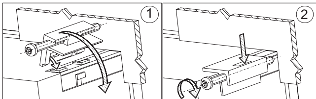
Fig.1. Controller fixing.
