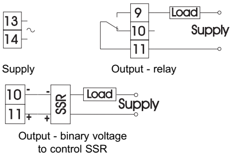
Fig.5. Connection of the supply and load circuit.
