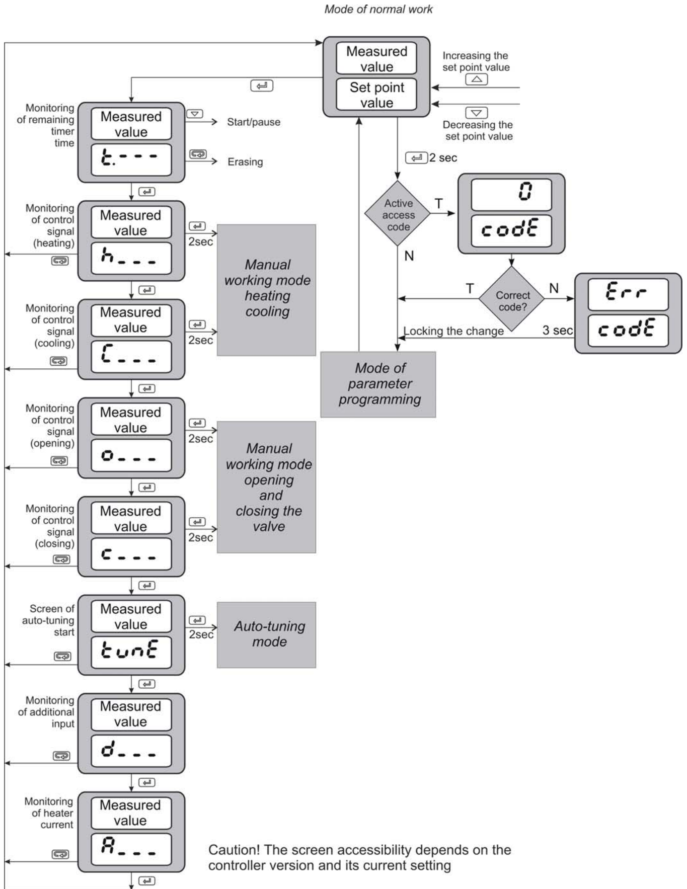
Fig. 13. Menu of controller service
