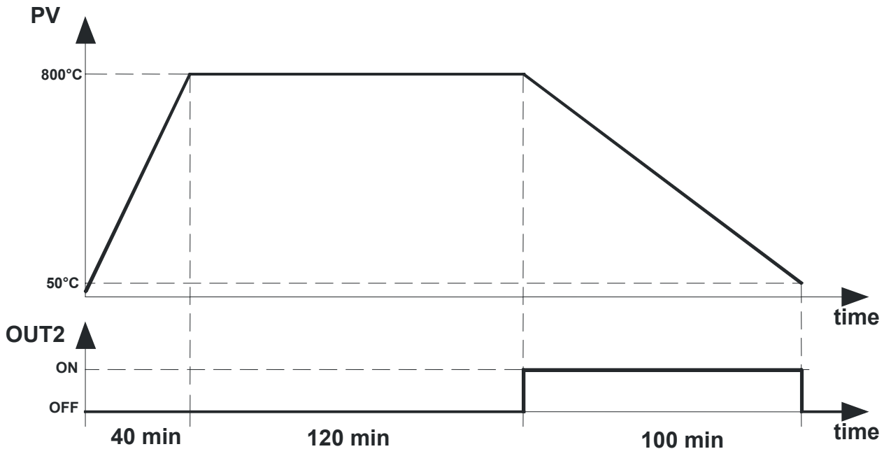
Fig. 23. Example of program
