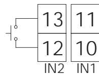
Fig. 8. Binary input 1 and 2
