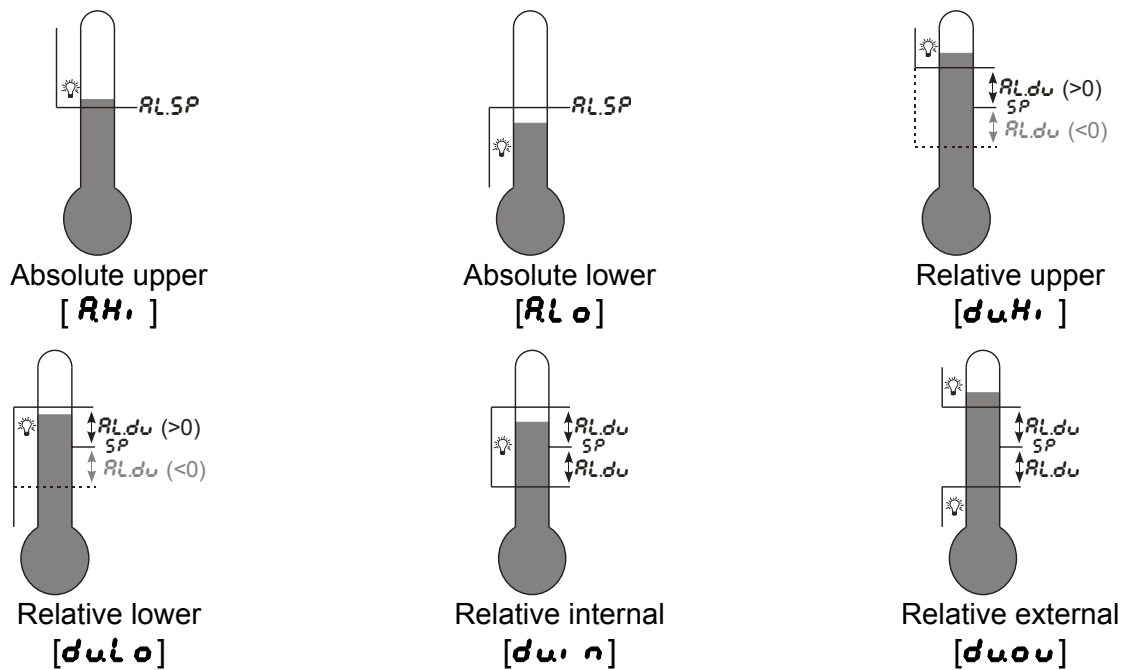
Fig. 22. Kinds of alarms
