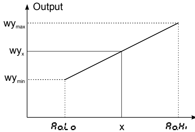
Fig. 24. Recounting of the signal for retransmission
