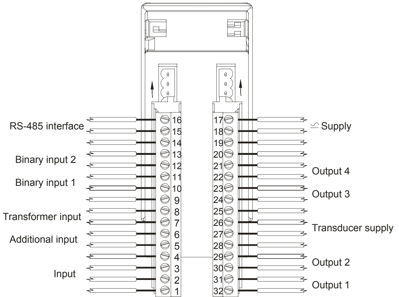
Fig. 3. View of controller connecting strips
