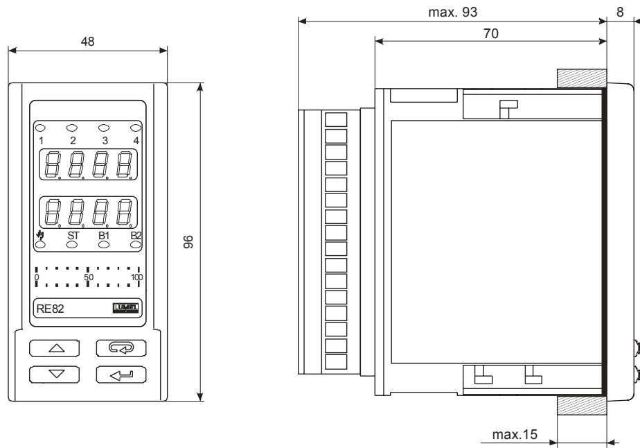
Fig. 2. Controller dimensions.
