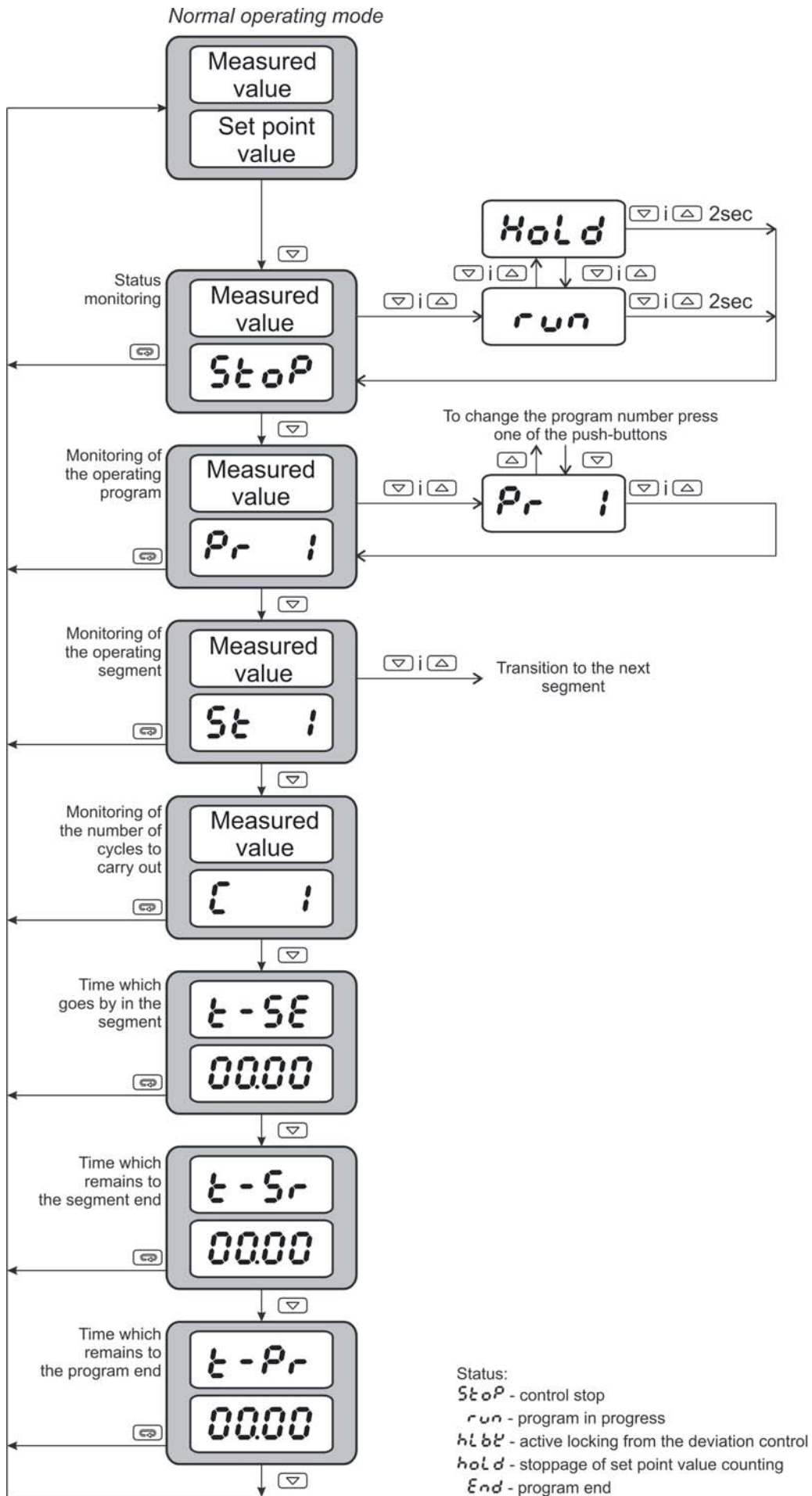
Fig. 27. Menu of programming control service
