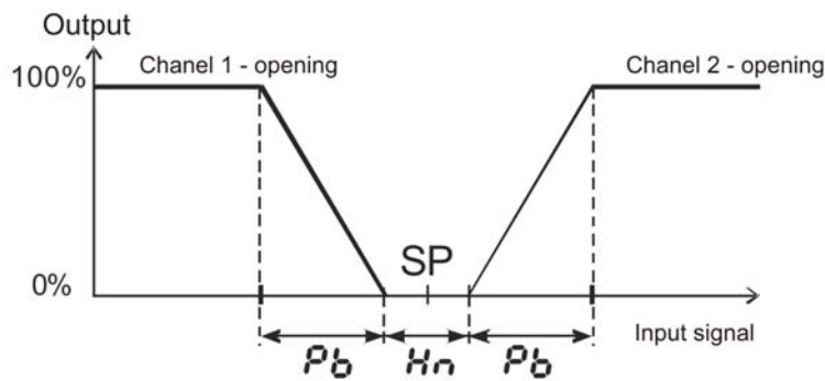
Fig. 18. three-stage step-by-step control
