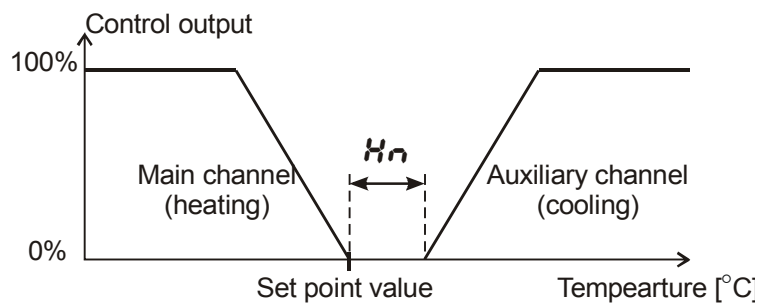
Fig.21. Control with two channels – heating-cooling type
