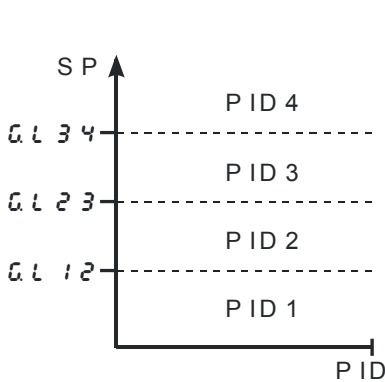
Fig. 19. "Gain Scheduling" switched over from SP
