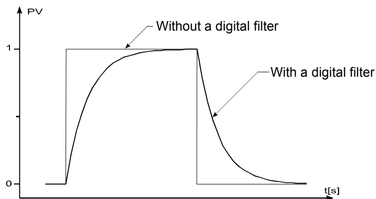
Fig. 25. Time characteristic of the filter
