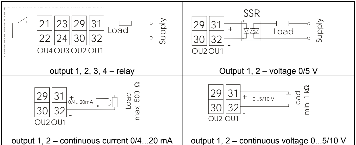
Fig. 7. Control outputs/alarm
