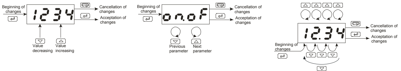
Fig. 15. Change of number , text and time parameter settings
