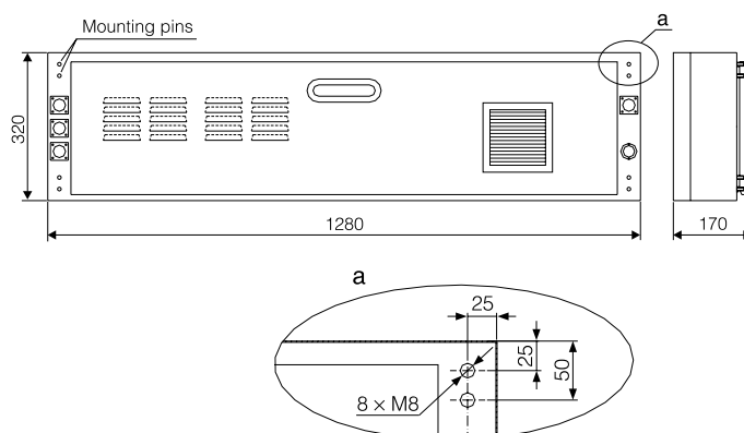
Fig. 1. Display overall dimensions and mounting pin spacing
