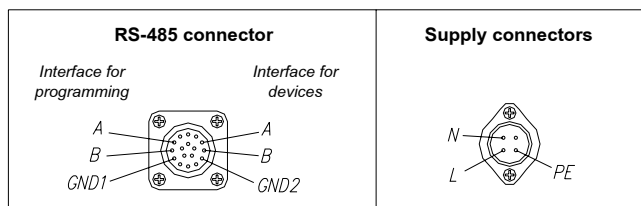
Fig. 3. Leads of signals on connectors.
