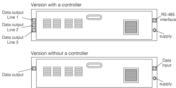
Fig. 2. Lay-out of connection sockets.
