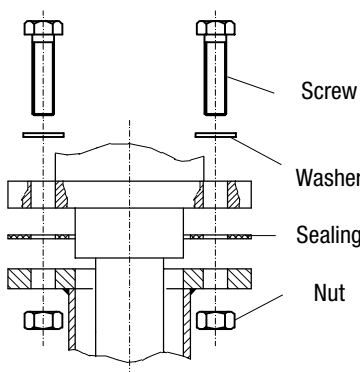
pos. 21 Mounting set Ø18
