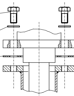
pos. 22 Mounting set M16
